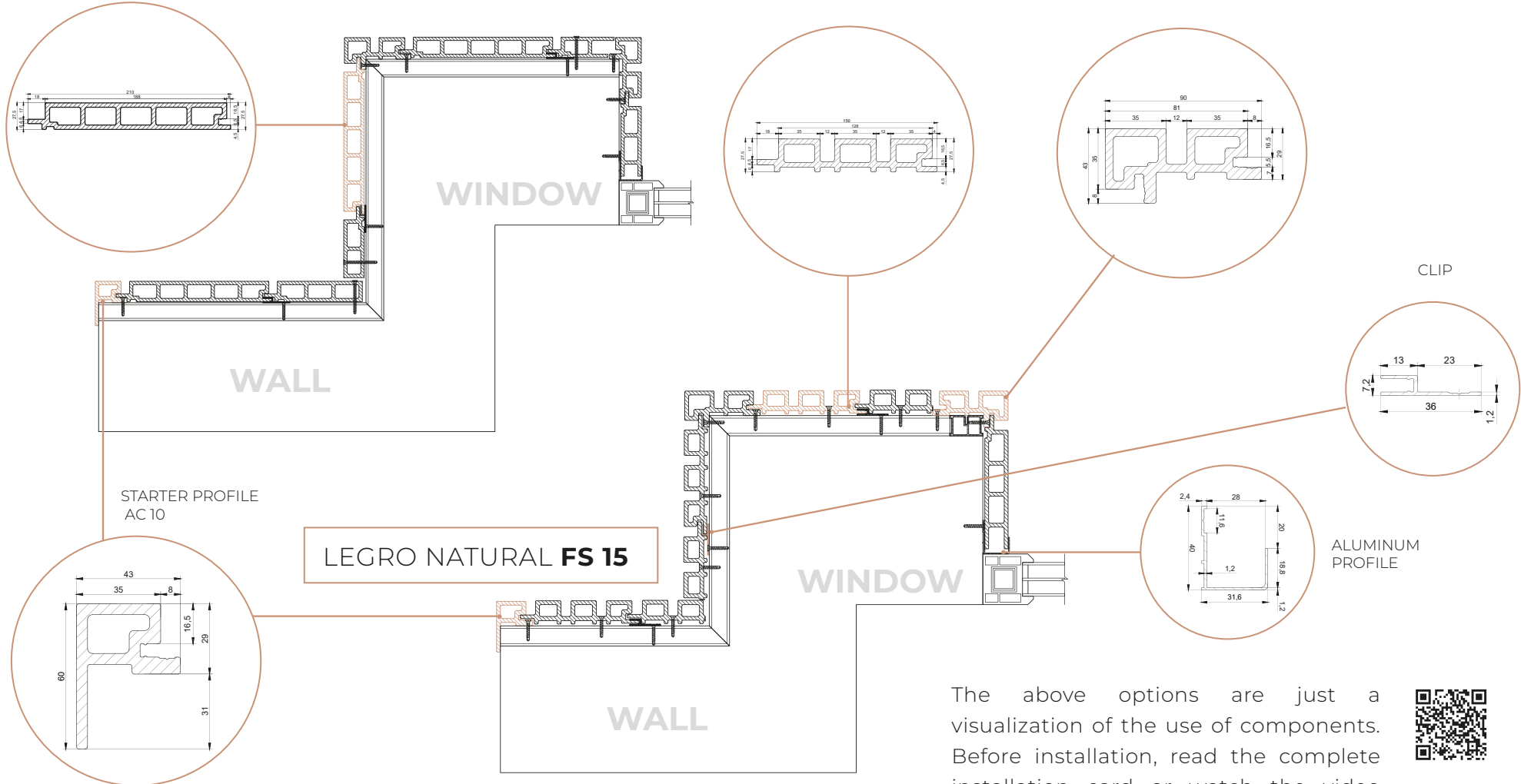
FACADE PROFILE FS 15
